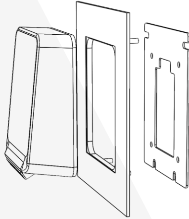
Figure 19: EVA Mounting
